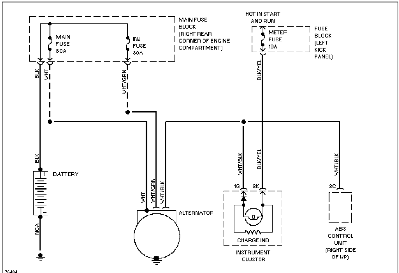
76434 Charging Circuit
